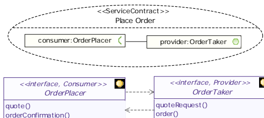
Figure 13: Service contracts models the business interfaces
