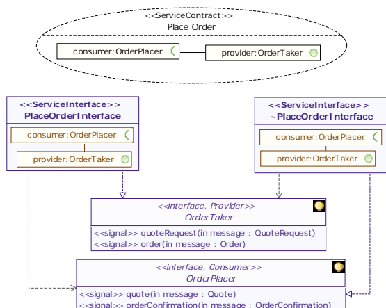
Figure 15: Service interfaces and service contracts are two different views
