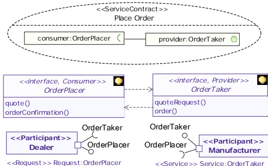
Figure 6: Specification of the Place Order service, consisting of two roles, their respective consumer and provider interface type, and the corresponding ports on the participants
